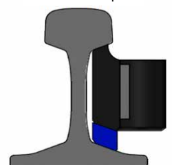
Vignol 60E1 with blue adapter
