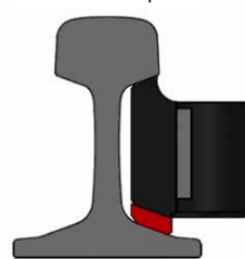
Vignol 54E2 with red adapter
